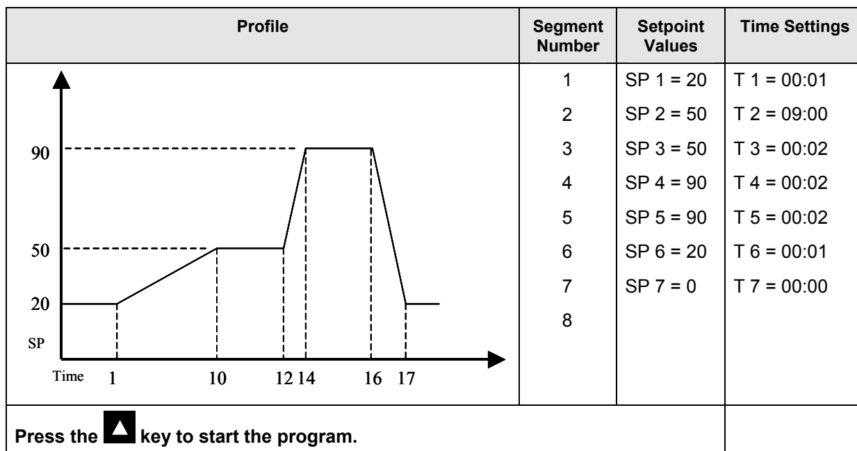
Figure 5-1 Program Example
